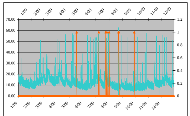
Influent MGD Peak Intensity/hr. Rain fall in./day South Prospect Street Activation NPDES# 033
