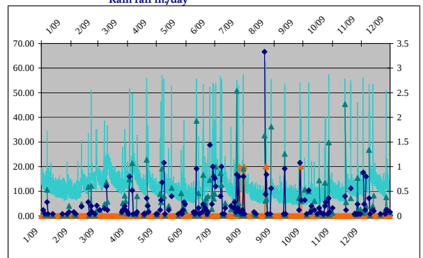
Influent MGD Main Street South Activation NPDES# 035 Peak Intensity/hr. Rain fall in./day
