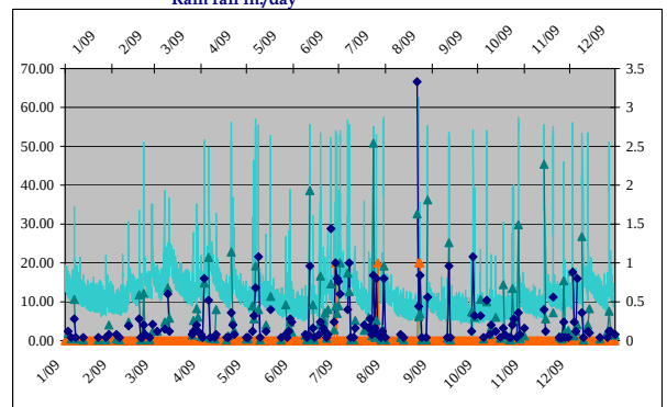
Influent MGD Peak Intensity/hr. Rain fall in./day Duncan Street Winter Street Activation NPDES # 021H
