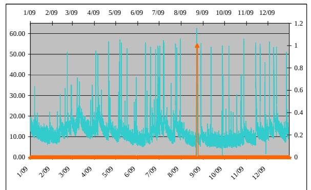
Influent MGD Peak Intensity/hr. Rain fall in./day
