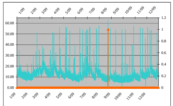
Influent MGD Peak Intensity/hr. Main Street North Activation NPDES# 019 Rain fall in./day
