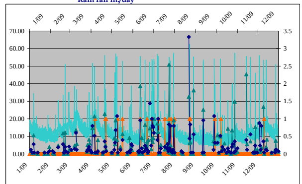
Influent MGD Middlesex Street Activation NPDES# 034 Rain fall in./day
