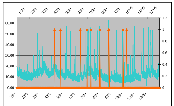
Influent MGD Peak Intensity/hr. Lower Siphon Activation NPDES# 013 Rain fall in./day
