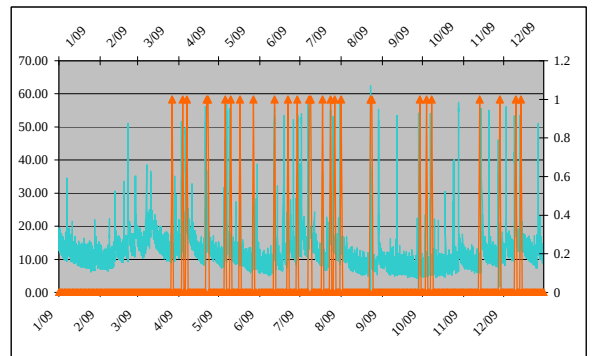
Influent MGD Peak Intensity/hr. Bradford Ave Activation NPDES# 032 Rain fall in./day
