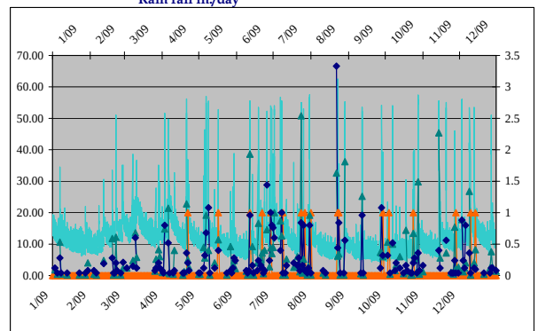
Influent MGD Peak Intensity/hr. Railroad Bridge Activation NPDES# 022 Rain fall in./day
