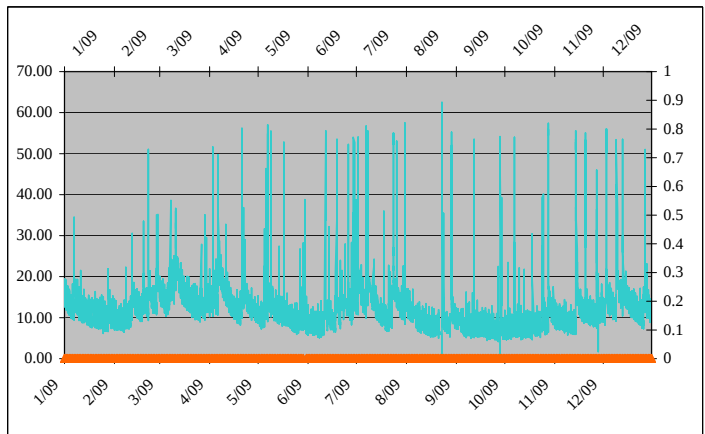
Influent MGD Peak Intensity/hr. Ferry Street Activation NPDES# 036 Rain fall in./day
