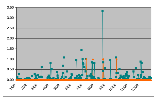
Influent MGD Front Street Activation NPDES# 031
