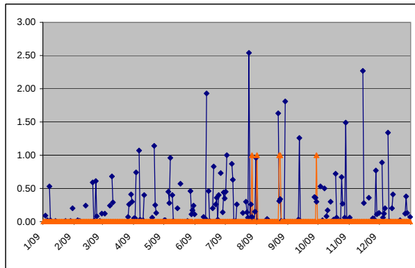
Rainfall (in./day) Peak Intensity/hr. Main Street South Activation NPDES# 035
