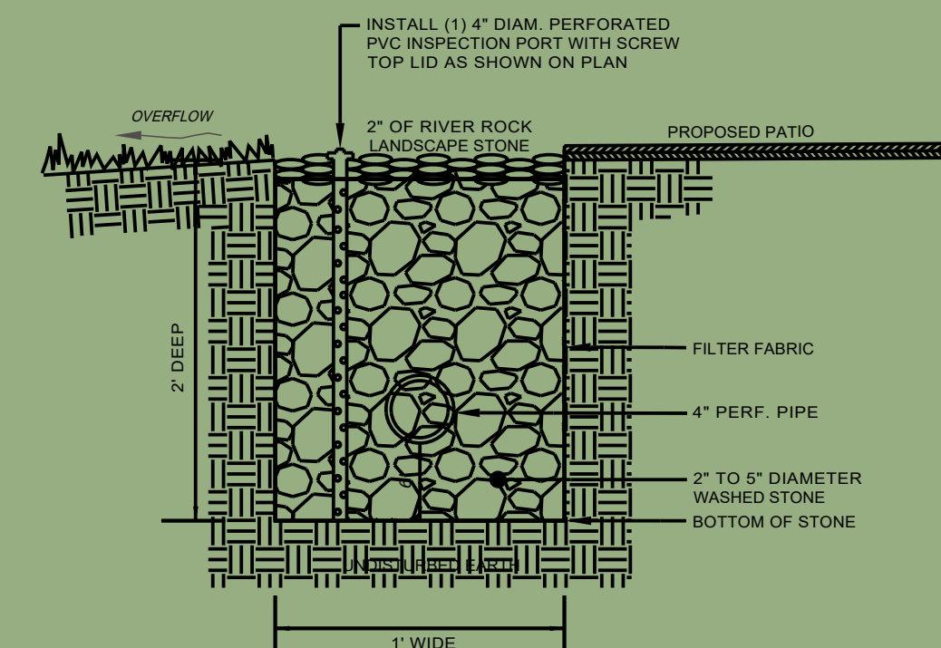
INFILTRATION TRENCH DETAIL (NOT TO SCALE)
