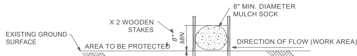
MULCH SOCK DETAIL (NOT TO SCALE)
